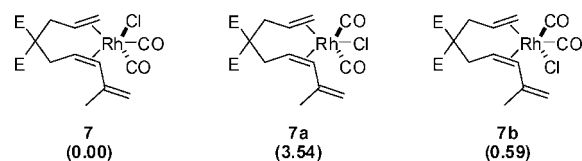
Figure 2. Possible \text{Rh}(\text{CO})_2\text{Cl} chlorine isomers during initial binding.
